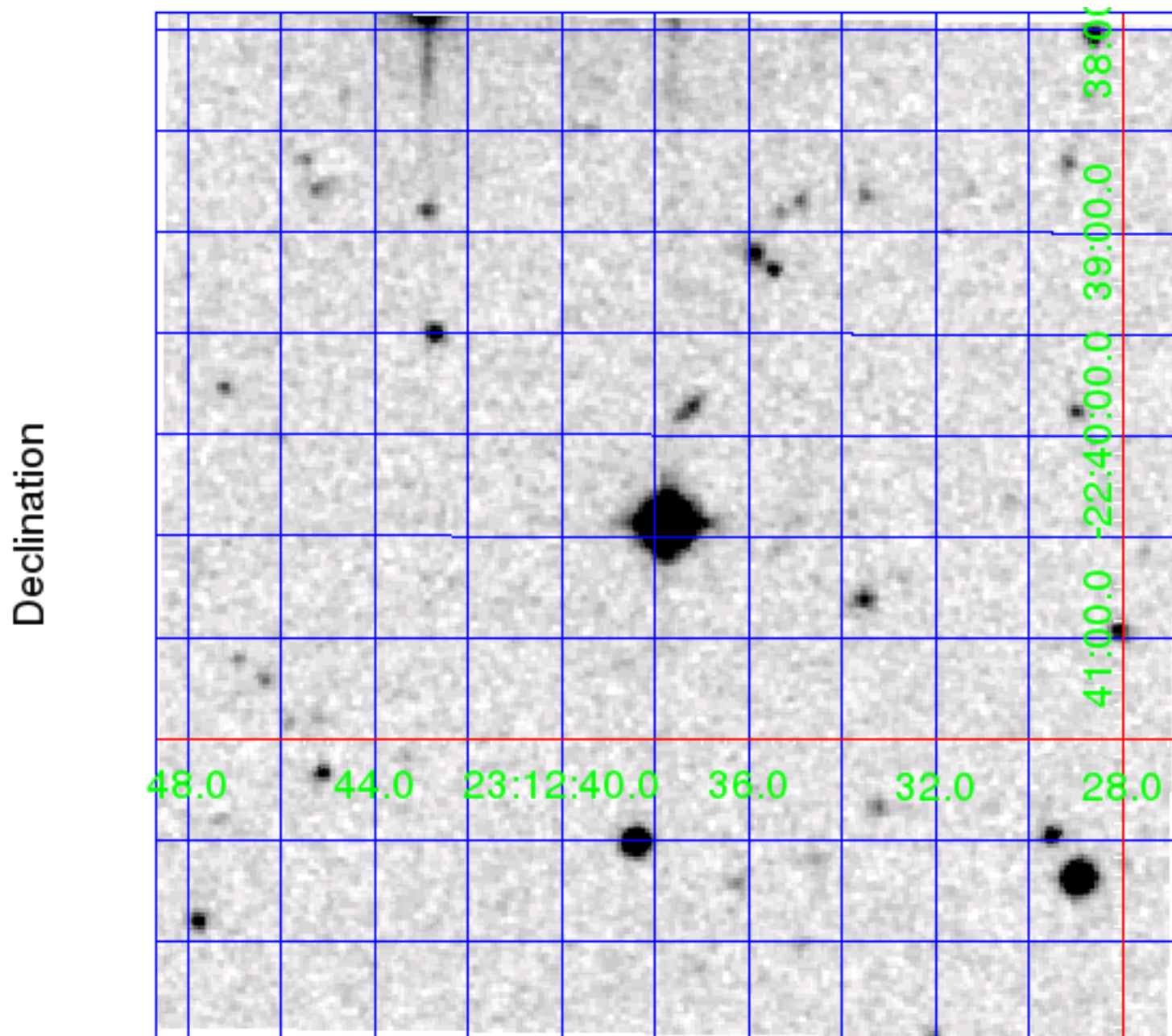
Digitized Sky Survey (DSS) red image. The 5' x 5' image is centered on the J2000 coordinates of target (204376737).
