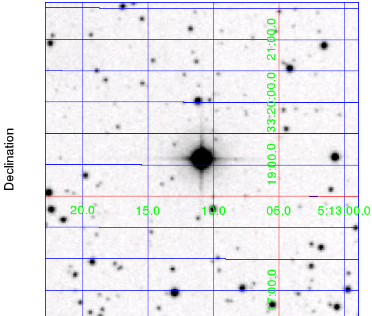
Digitized Sky Survey (DSS) red image. The 5' x 5' image is centered on the J2000 coordinates of target (367366318).
