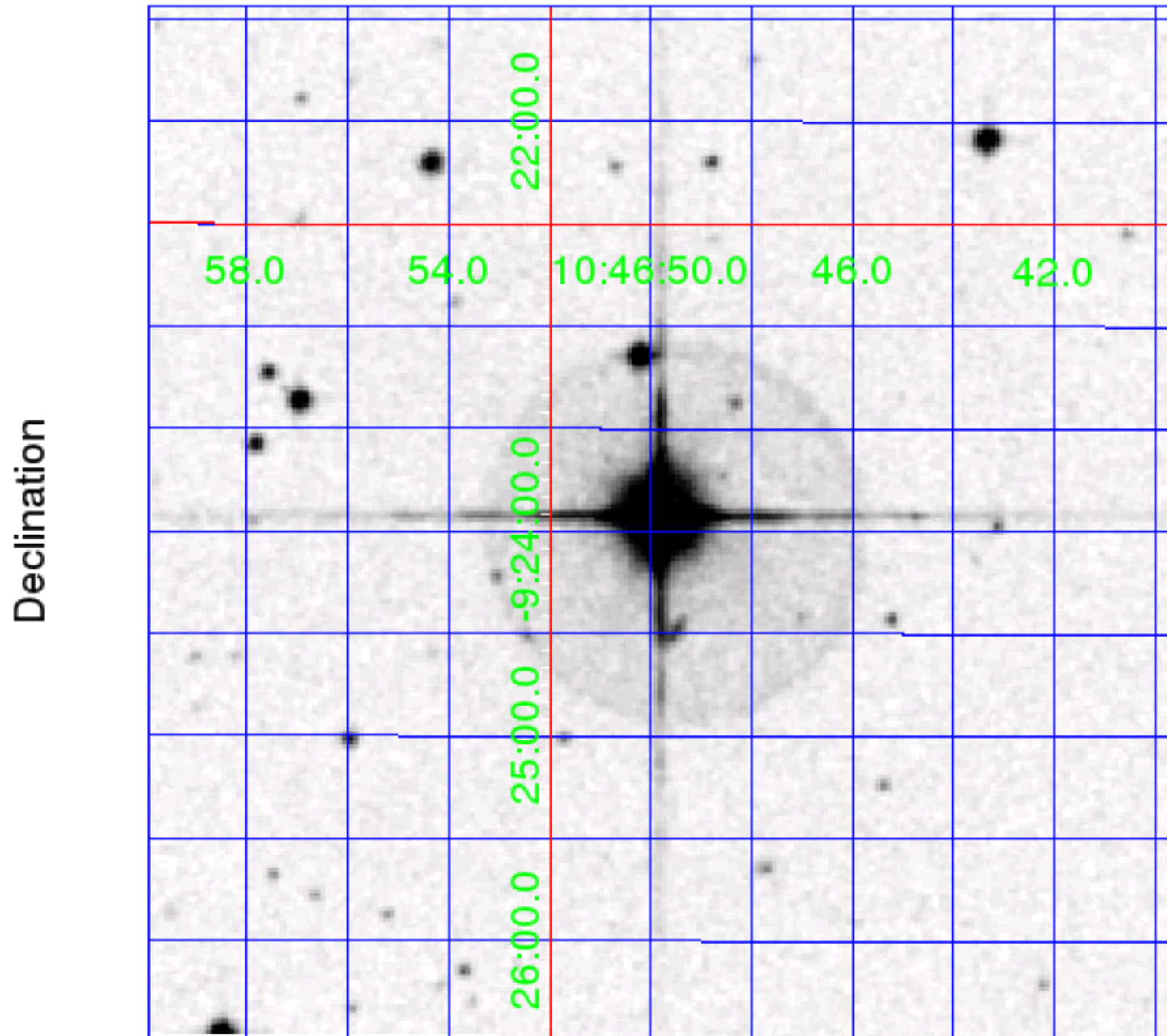
Digitized Sky Survey (DSS) red image. The 5' x 5' image is centered on the J2000 coordinates of target (55092869).
