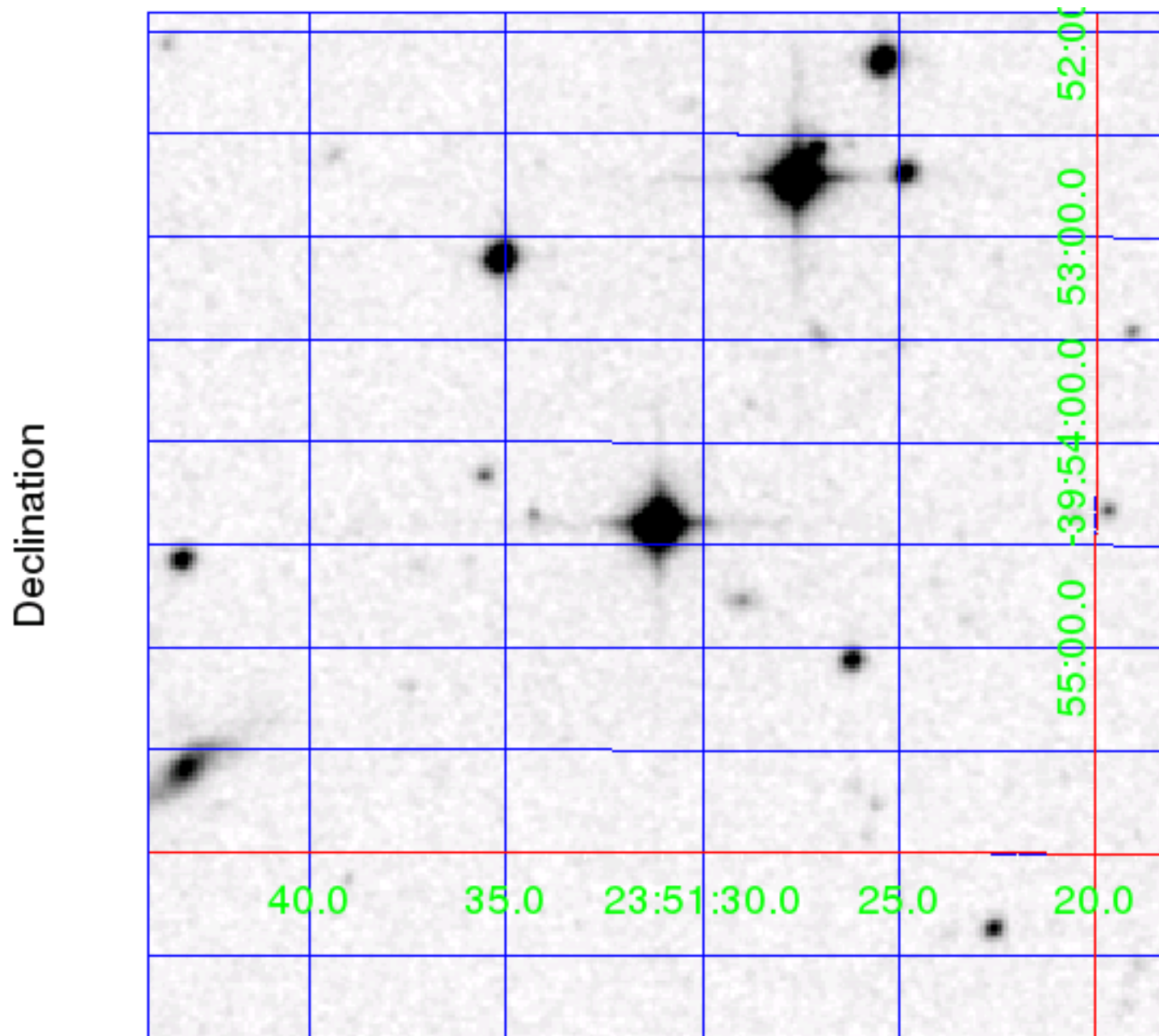
Digitized Sky Survey (DSS) red image. The 5' x 5' image is centered on the J2000 coordinates of target (183537452).
