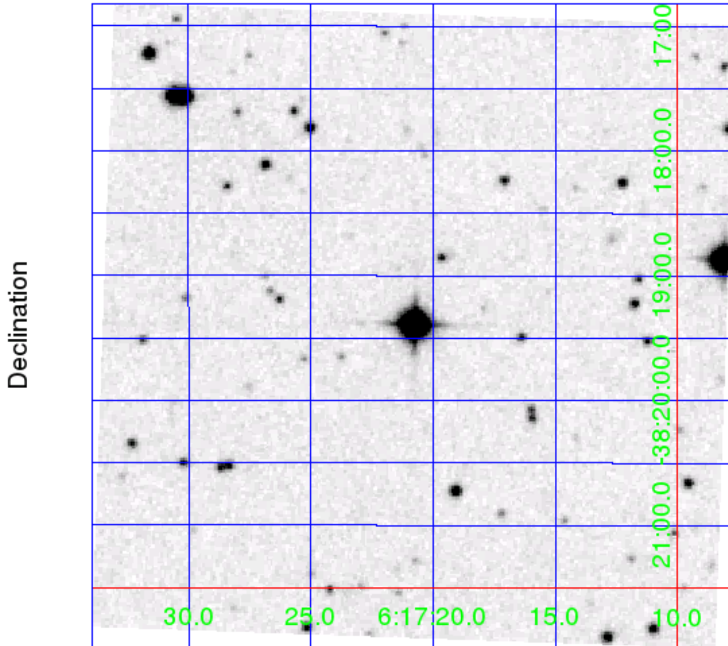
Digitized Sky Survey (DSS) red image. The 5' x 5' image is centered on the J2000 coordinates of target (393414358).
