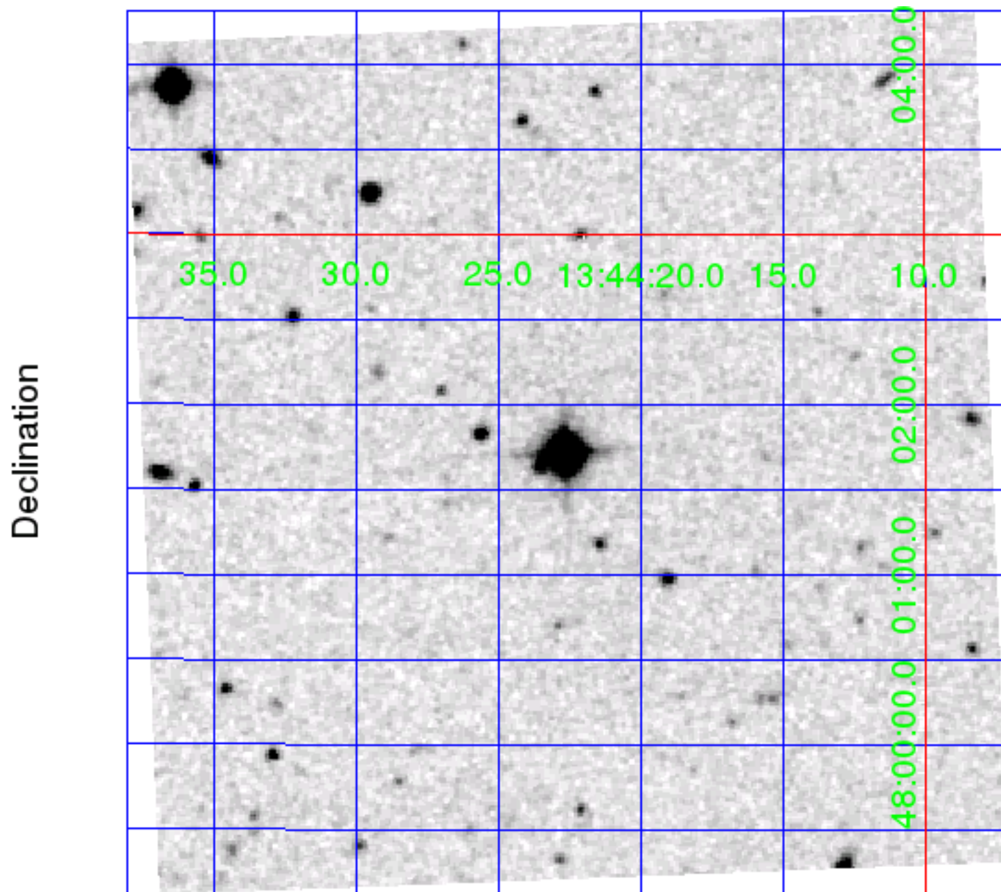
Digitized Sky Survey (DSS) red image. The 5' x 5' image is centered on the J2000 coordinates of target (311035838).
