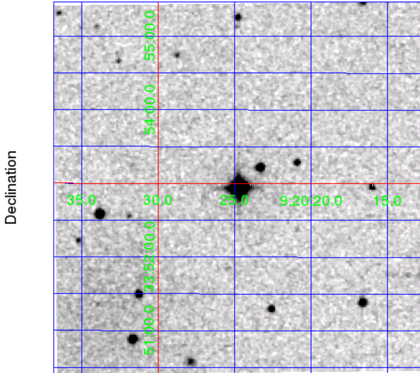
Digitized Sky Survey (DSS) red image. The 5' x 5' image is centered on the J2000 coordinates of target (8767448).
