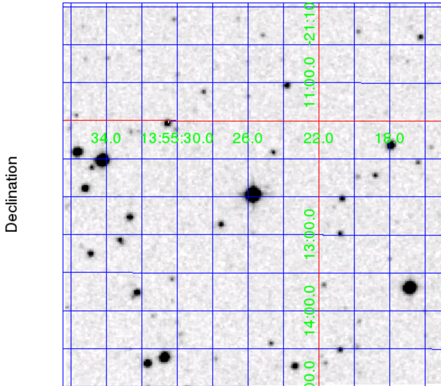
Digitized Sky Survey (DSS) red image. The 5' x 5' image is centered on the J2000 coordinates of target (220029715).
