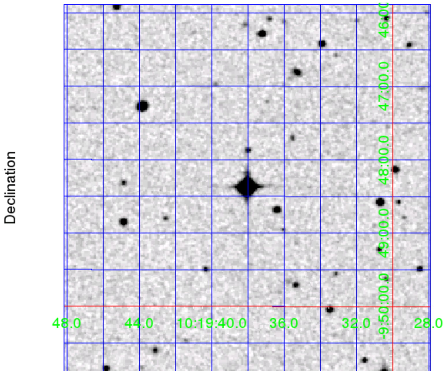
Digitized Sky Survey (DSS) red image. The 5' x 5' image is centered on the J2000 coordinates of target (36734222).
