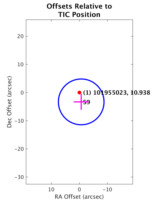
Planet Candidate 1
