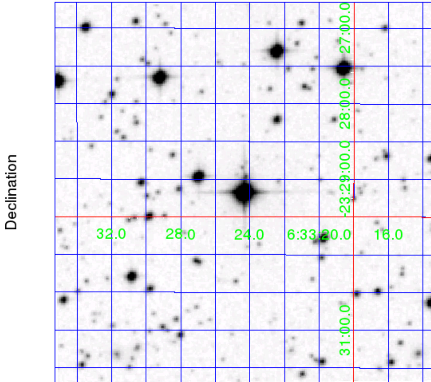
Digitized Sky Survey (DSS) red image. The 5' x 5' image is centered on the J2000 coordinates of target (47911178).
