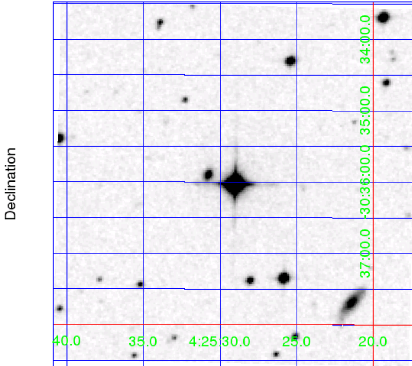
Digitized Sky Survey (DSS) red image. The 5' x 5' image is centered on the J2000 coordinates of target (170634116).
